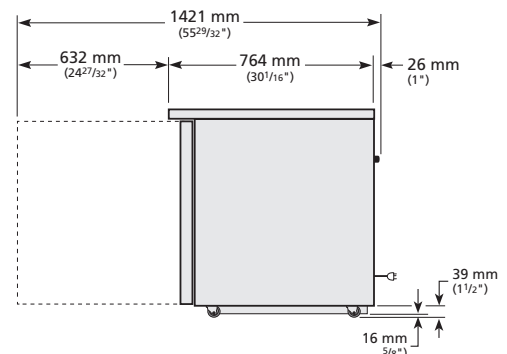
RIGHT VIEW
